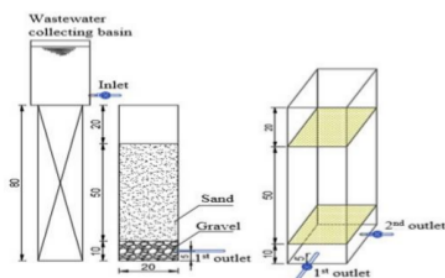
Figure 2. Schematic diagram of the biofilter.
