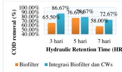
Figure 5. The efficiency of COD removal.
