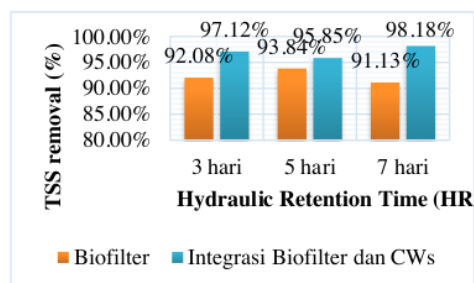
Figure 6. The removal efficiency of TSS.
