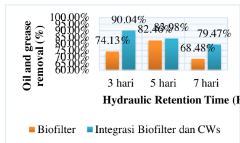
Figure 7. Efficiency removal of oil and grease.
