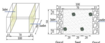
Figure 3. Schematic diagram of the HSSFCW.
