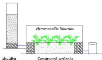
Figure 4. Schematic diagram of combined biofilter dan HSSFCW.
